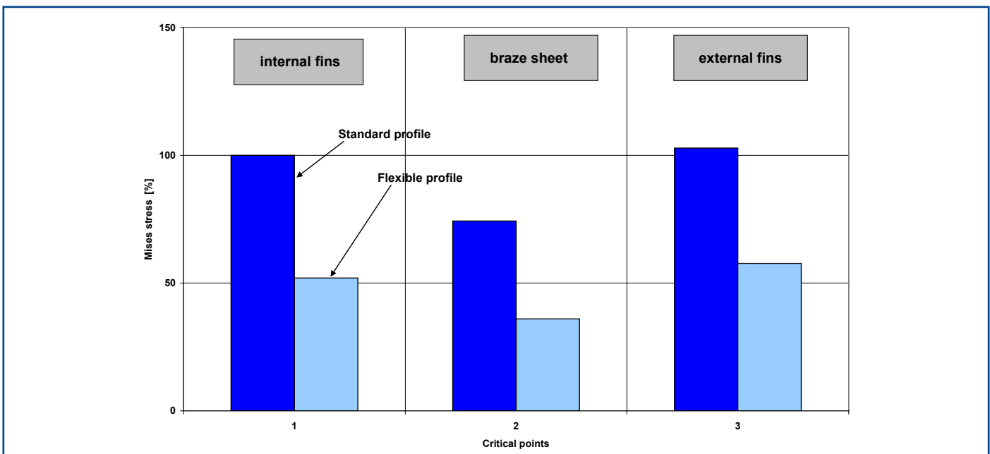
Cooler with flexible profile
